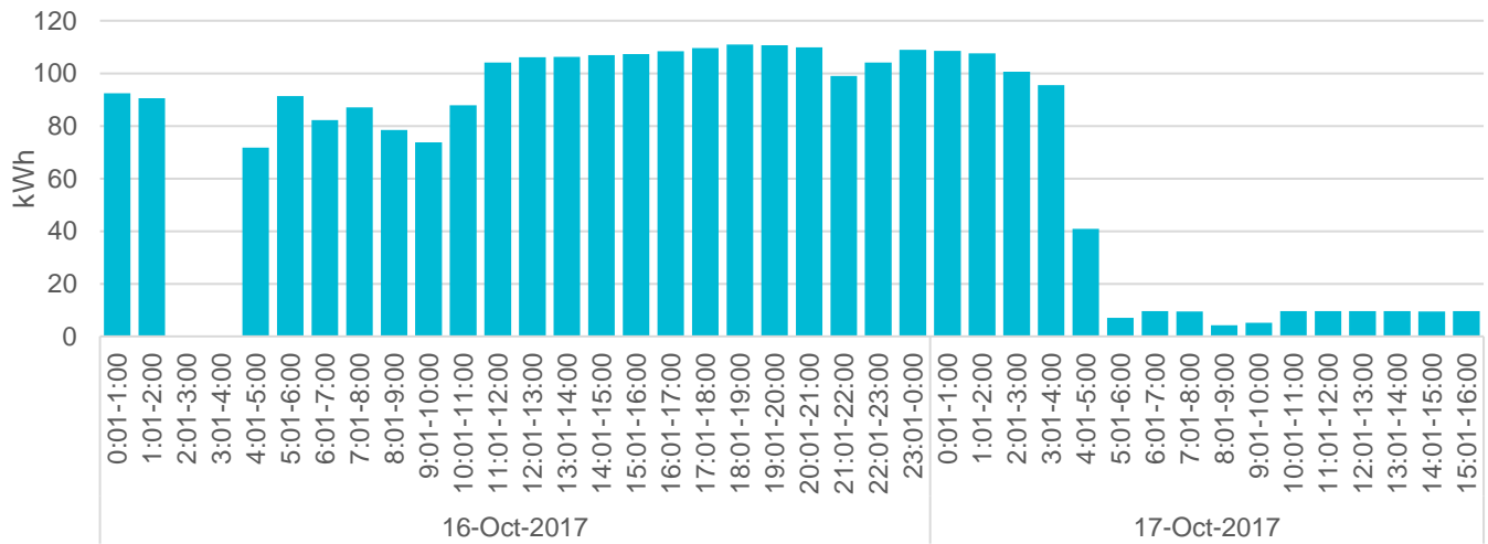
Figure H-1: Hourly power consumption
